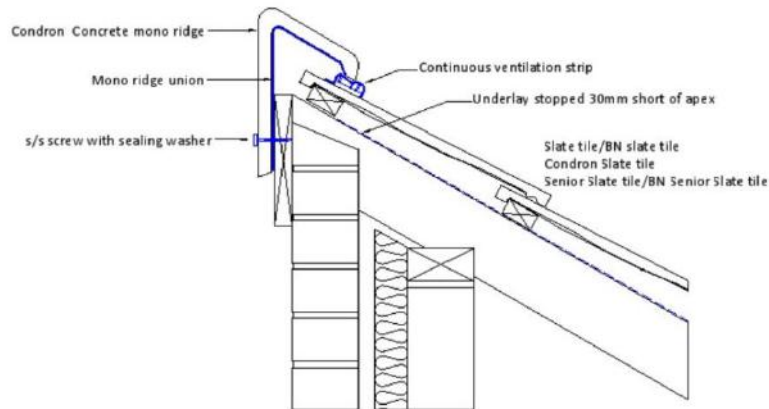
Dry fix mono ridge detail with Concrete Senior slate tiles
