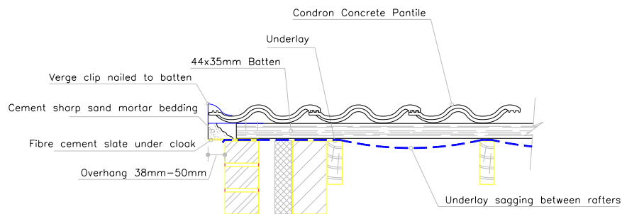
Mortar Bedded Verge
