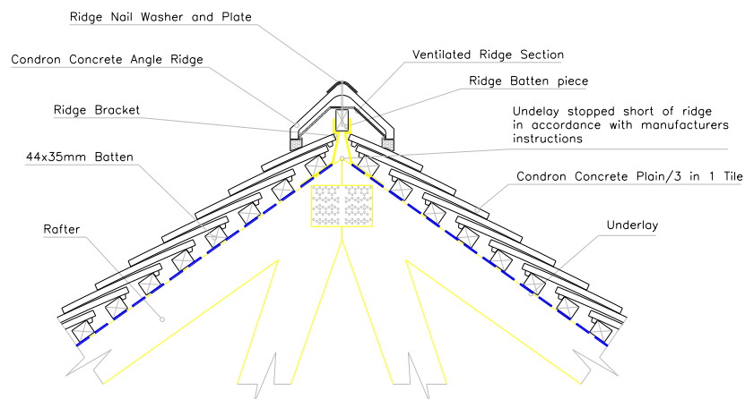
Dry Ridge System (Plain Tile / 3 in 1 Tile)
