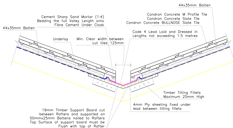
Lead Valley
