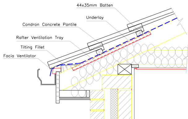
Eaves Ventilation/Pantile
