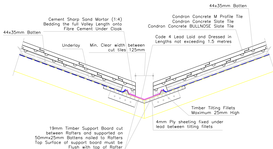
Lead Valley
