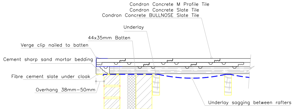
Mortar Bedded Verge
