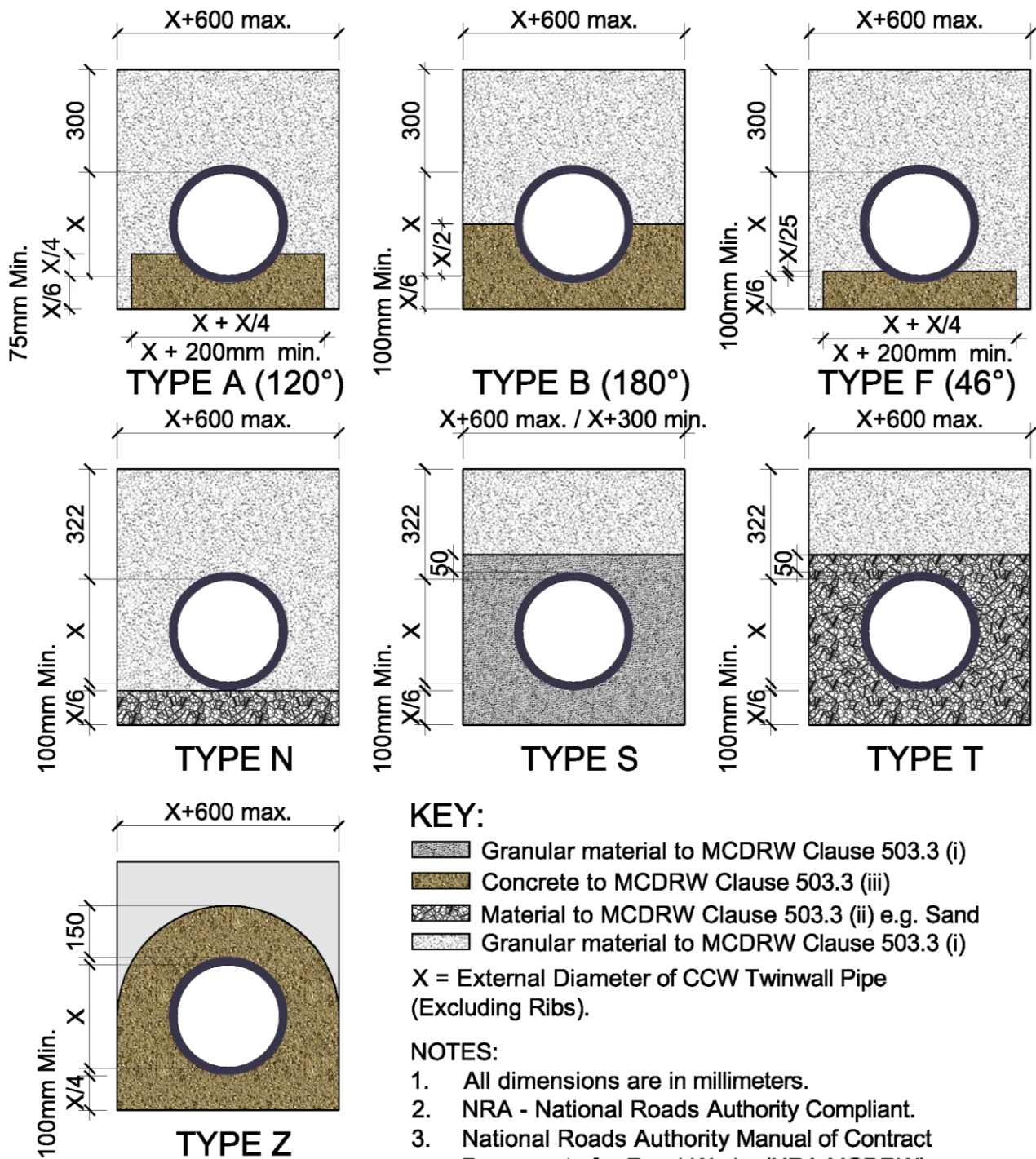
Figure 4: Surface Water Drain Trench and Bedding Details
