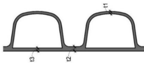
Typical Pipe Corrugation Profile
